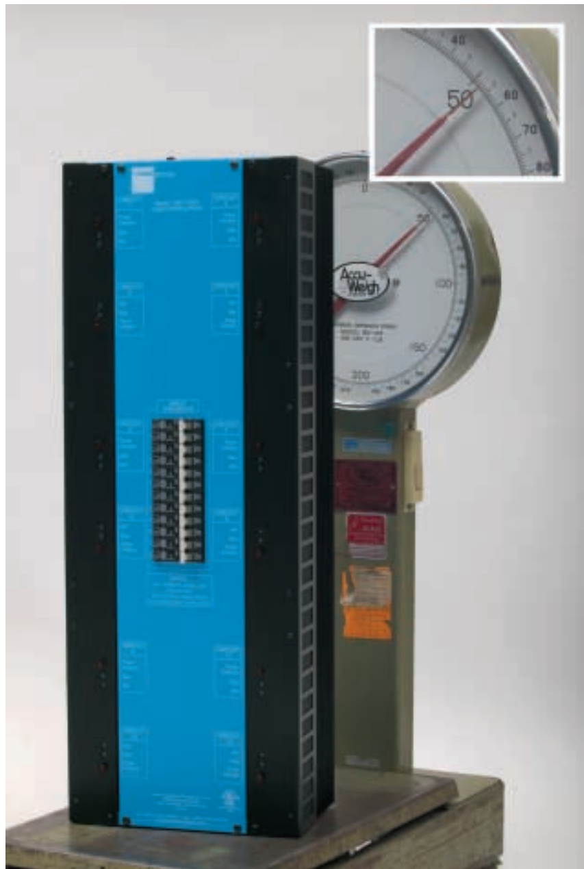
The SSD-12/20 weighs 53 pounds.
